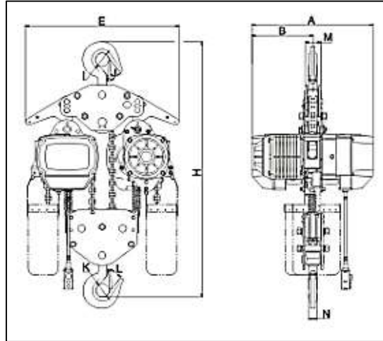
Hoist Dimensions
