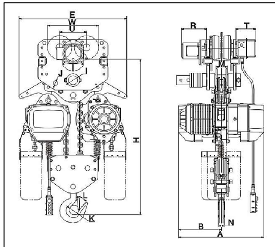
10 Ton Hoist with Motorized Trolley
