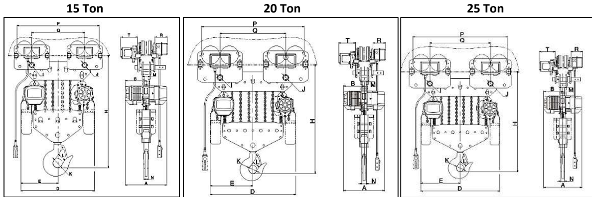
Hoist Dimensions
