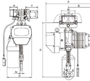
Hoist with Motorized Trolley Dimensions (in inches)
