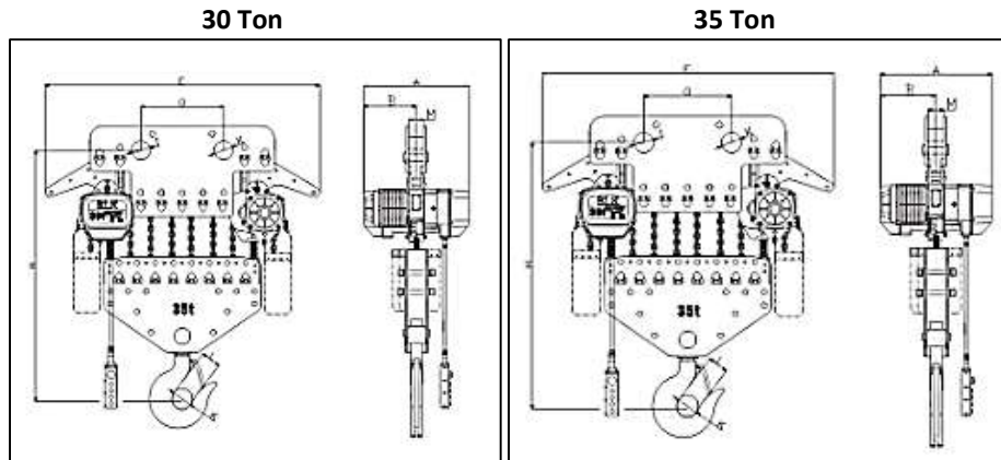
Hoist Dimensions
