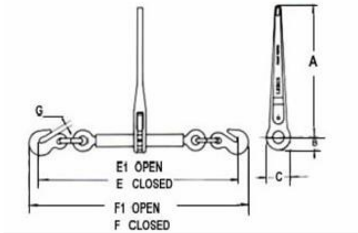
SPECIFICATIONS – TABLE 1 Binder Load Ratchet with Grab Hook
