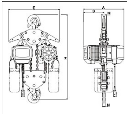
Hoist Dimensions
